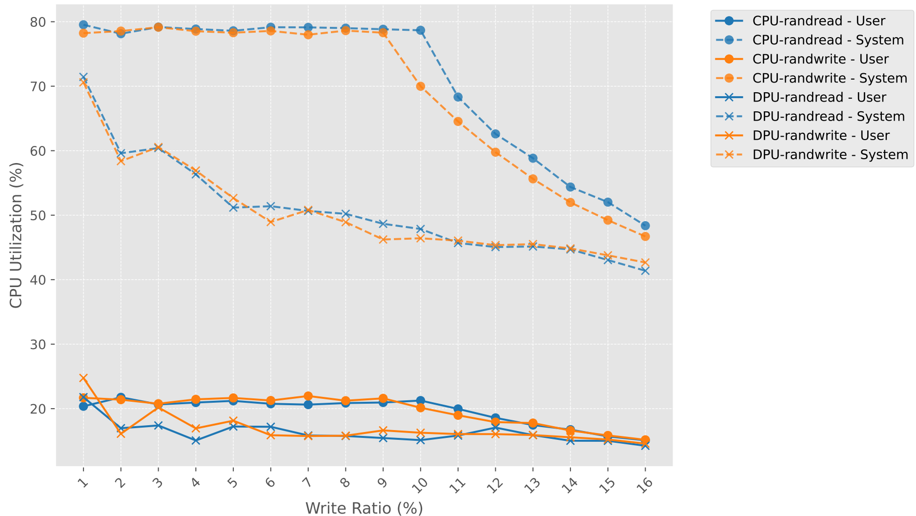
CPU Utilization vs Write Ratio (numjobs)
